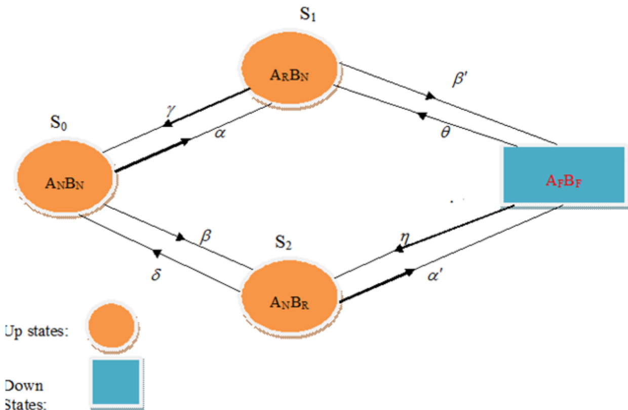
State Transition Diagram for the first System
