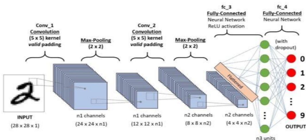
Fig 1. Architecture of the Two-Layer Convolutional Neural Network with Fully Connected Layers
