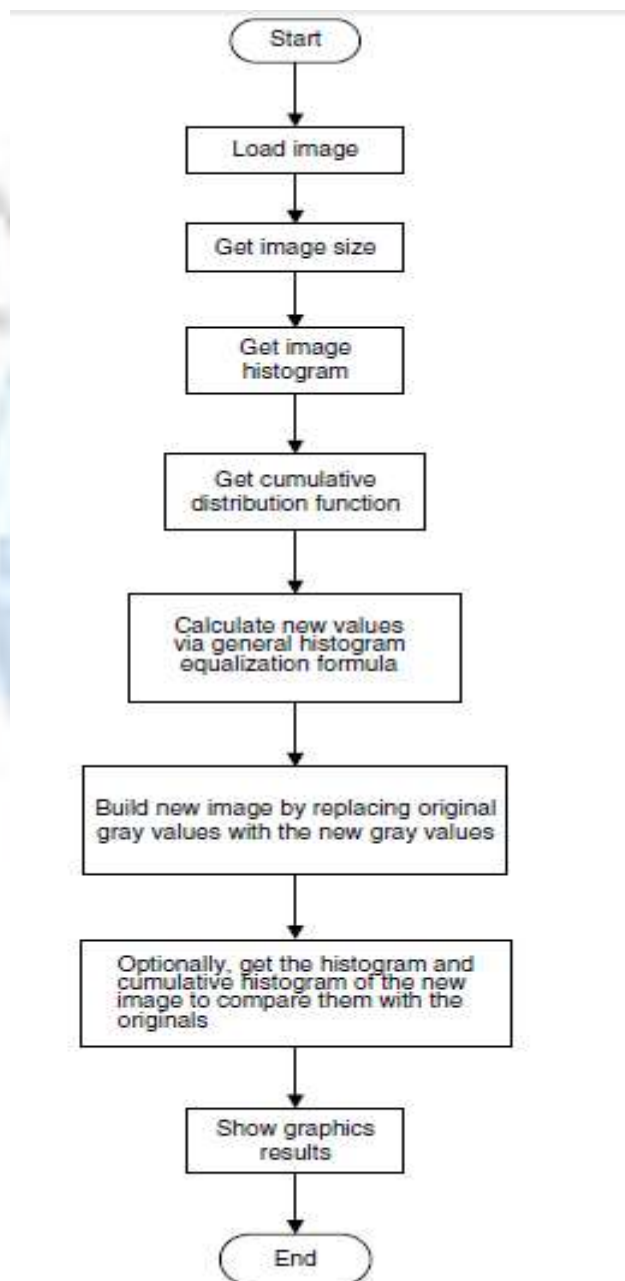
Figure 4: Algorithm implemented
