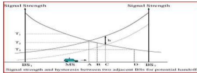
Figure7. Handover threshold
