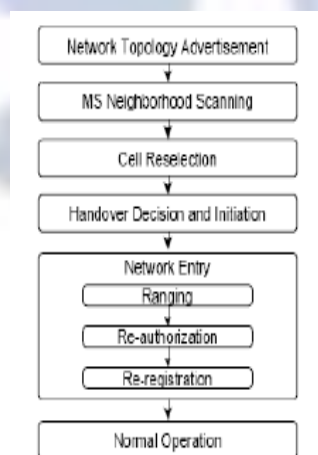
Figure3. Handover process
