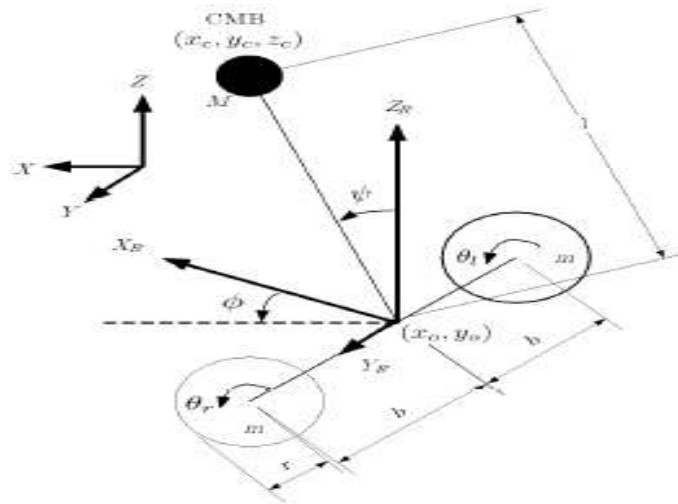
Figure 1: Dynamic Model of Self-Balancing Robot [10]
