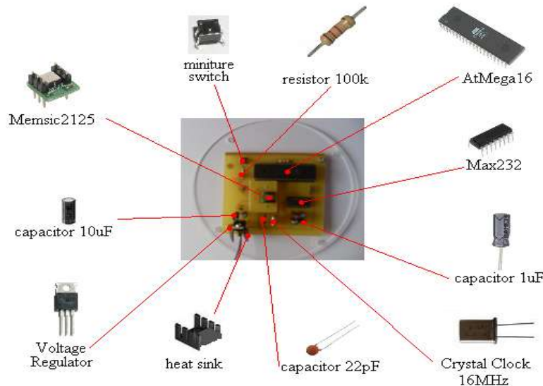
Figure 8: Control Sub-system
