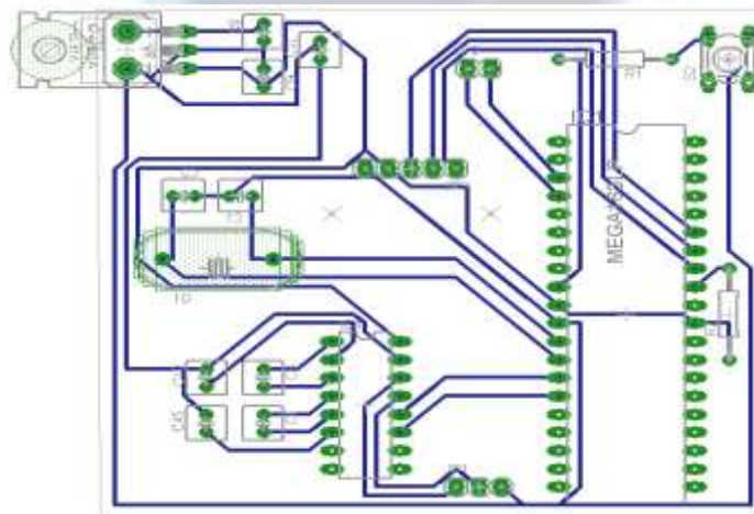
Figure 6: PCB layout for circuit
