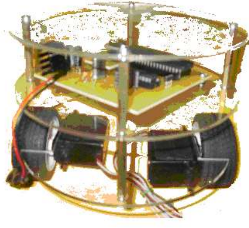
Figure 7: Self-Balancing Robot
