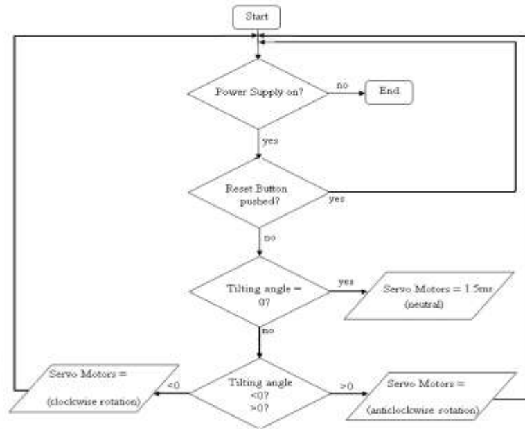
Figure 9 Functional diagram
