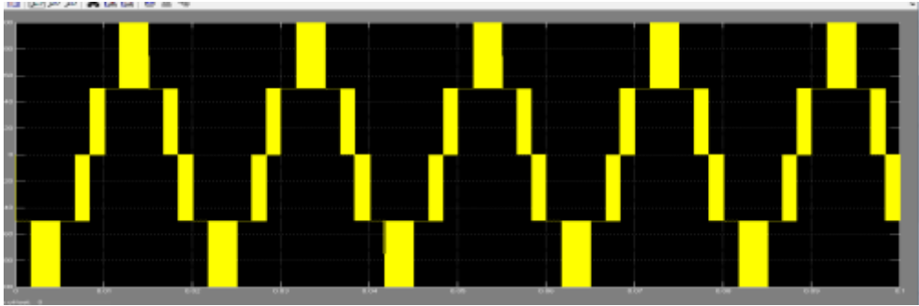
Figure 5: five level output voltage at load side
