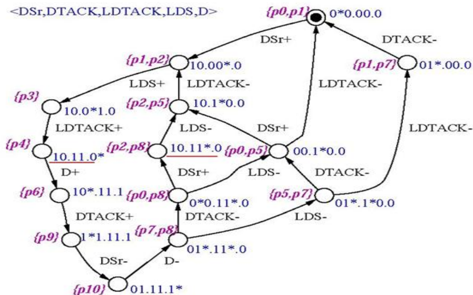
Fig. 4: State graph for the Read cycle
