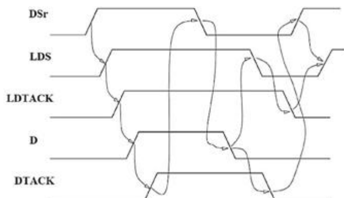
Fig. 2: Read Cycle
