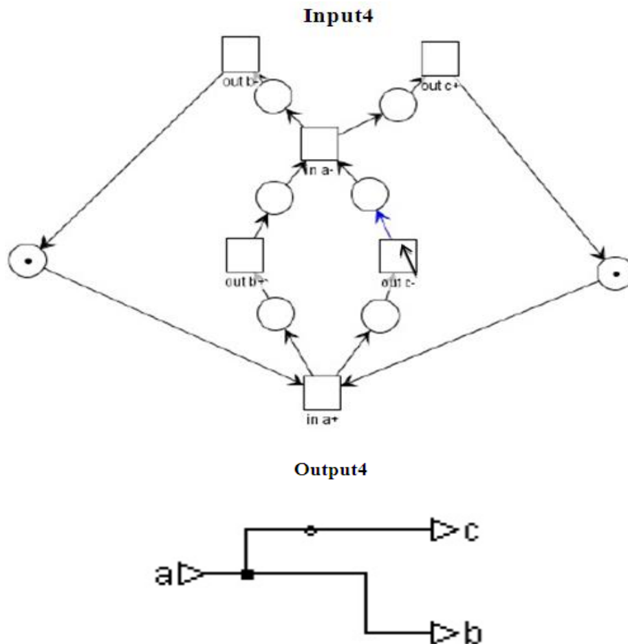
Fig. 11: Circuit generated by using Petri Net
