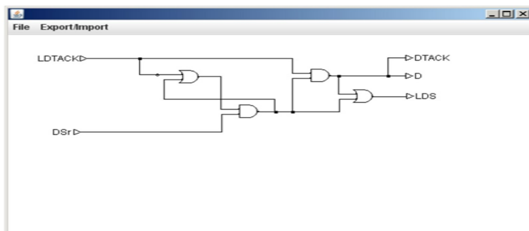
Fig. 10: Generated logical circuit
