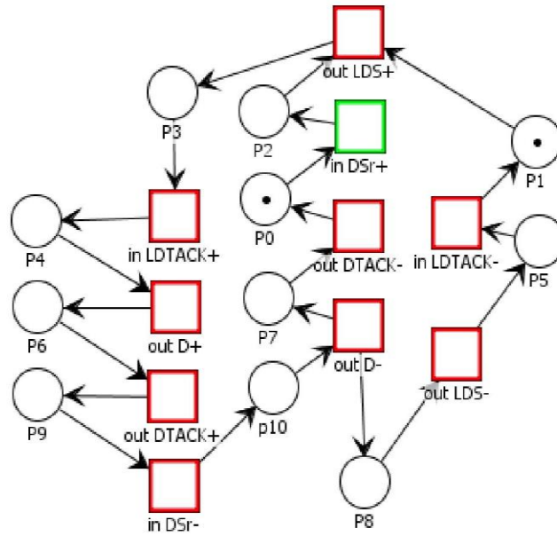
Fig. 3: Signal Transition Graph
