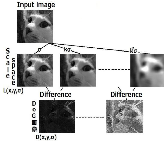
Figure 1: Calculation Flow of DoG Image
