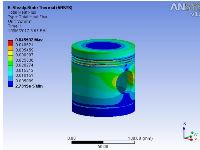
Figure 11 Total Heat Flux
