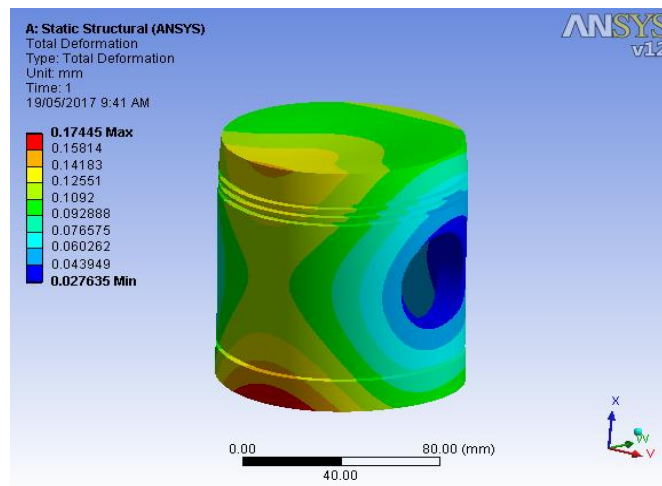
Figure 9 Total Deformation
