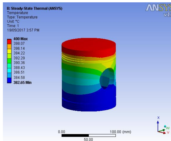
Figure 10 Temperature Distribution
