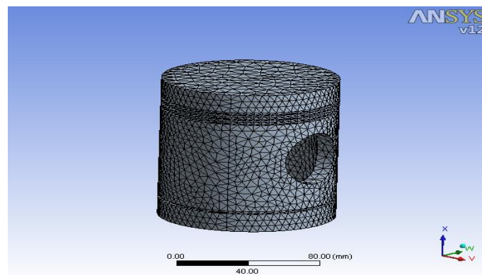
Figure 5 Meshed model of Piston in ANSYS workbench
