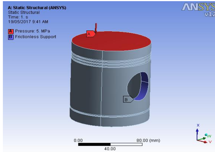
Figure 6 Applied Static constraints on Piston
