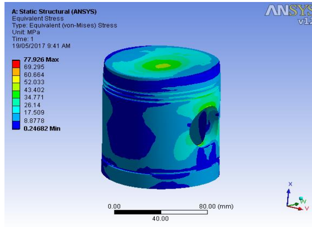
Figure 8 Equivalent (von-mises) stress
