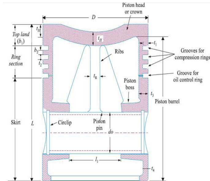
Figure 1: Piston Nomenclature
