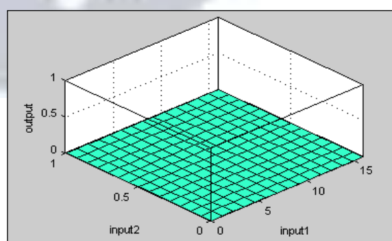
Fig 2.3: Surface Viewer
