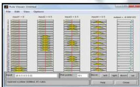
Fig 2.2: 81 Rules Generated
