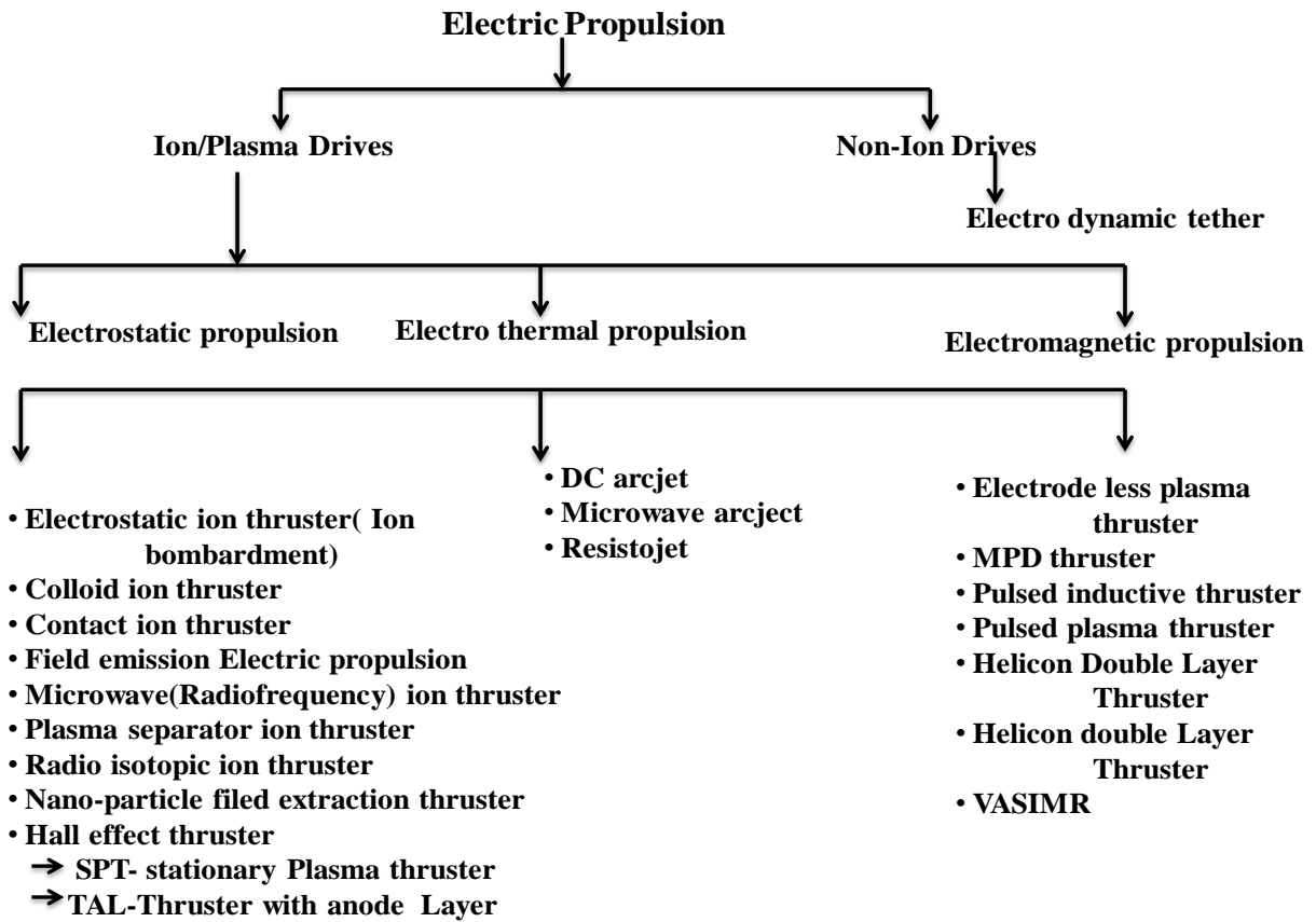
Figure 1. Broad classification of Electric Propulsion (EP) technologies
