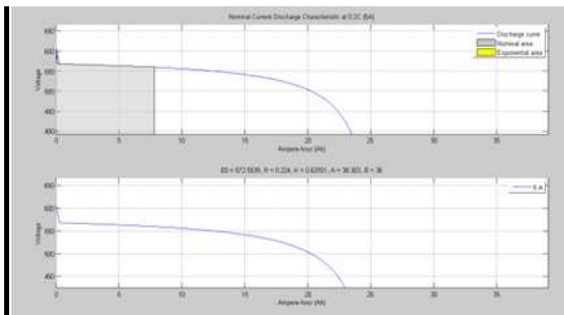
Fig 5. Lead-acid battery characteristics
