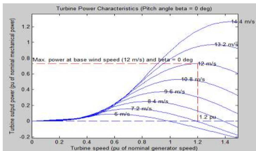
Fig 3. Wind Turbine Speed-Power Characteristics
