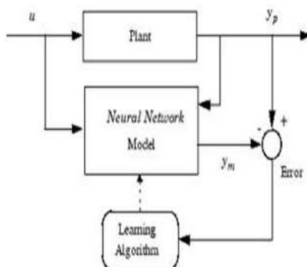
Fig 6. Block diagram of Narma - L2 controller
