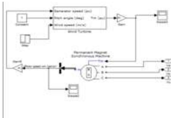
Fig 2.Subsystem Implementation of the WT model
