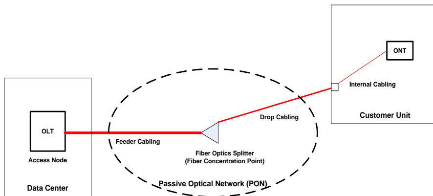
Figure 7. Structure of Access Network
