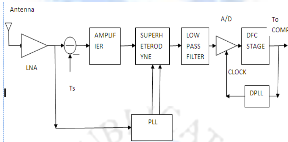
Figure 1: Block diagram of CW Radar Receiver. Ts is the transmitted signal.
